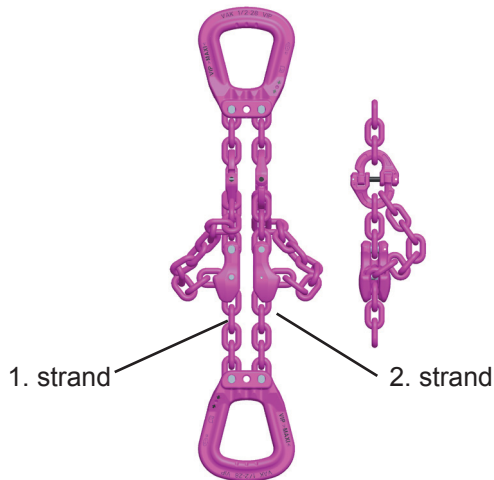
Pic. 10: Exposure shows parallel 2-leg-sling. Identical strand length when shortened
