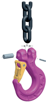
Pic. 6: Assembly system
