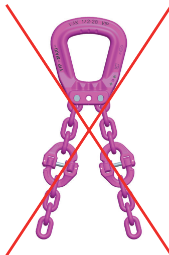
Pic. 13: Wrong assembly of connection links
