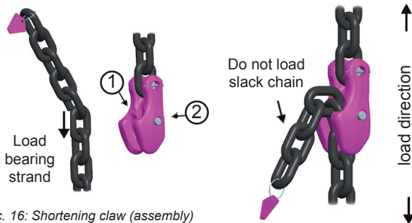
Pic. 16: Shortening claw (assembly)
