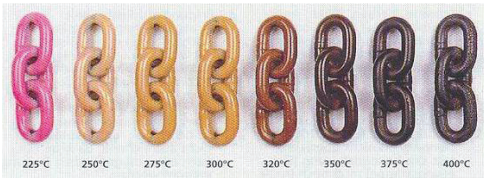
Pic. 5: Patented VIP overheating indicator for pink powder coated chains
