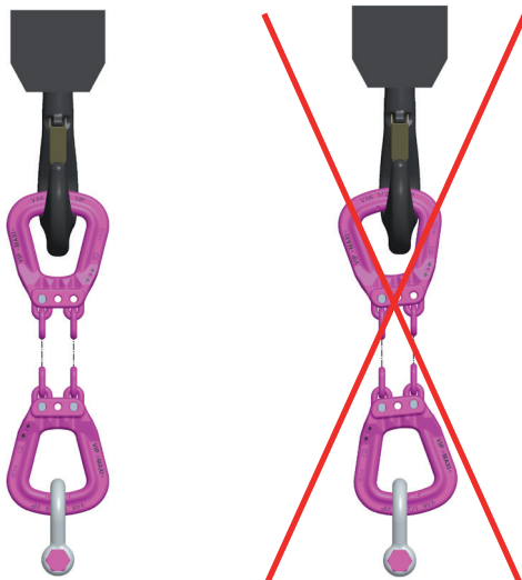
Pic. 11: Required centric resp. wrong (excentric) position
